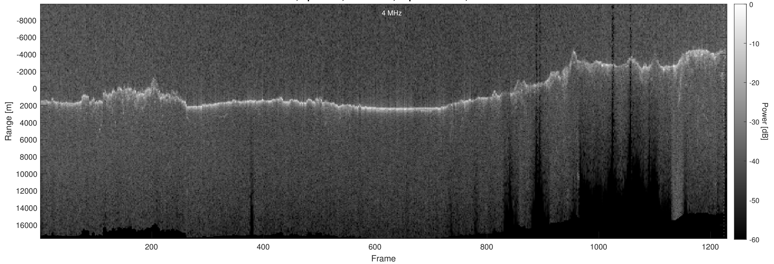
Orbit 5136, Optimized, No Window, Depth-Corrected, Channel 2
