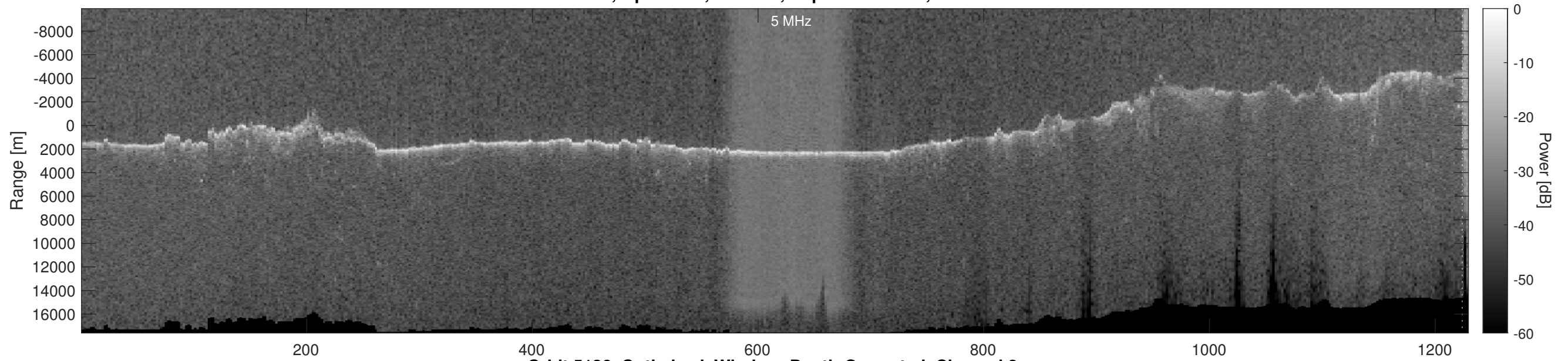
Orbit 5136, Optimized, Window, Depth-Corrected, Channel 2
