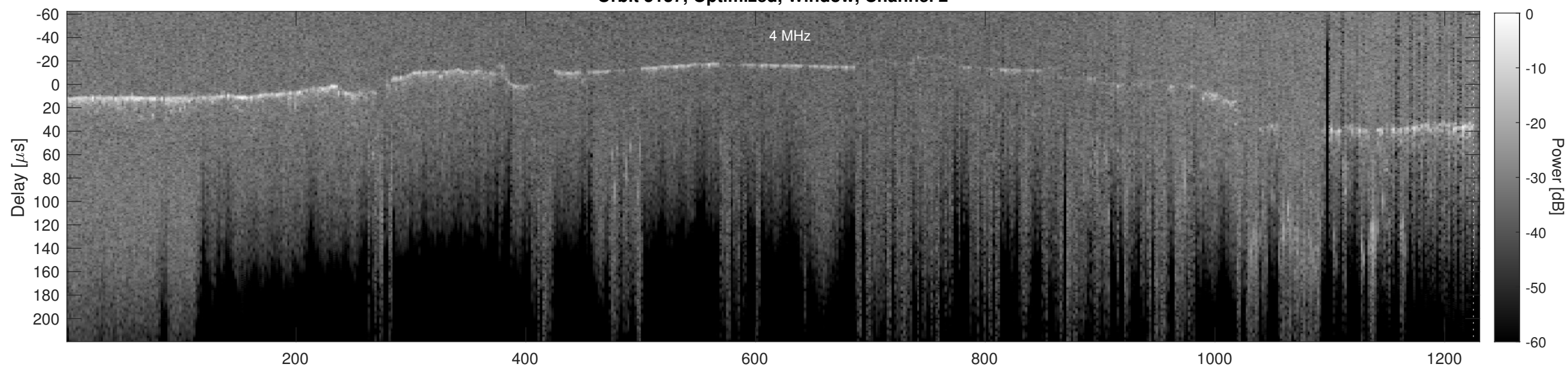
Orbit 5137, Cluttergram
