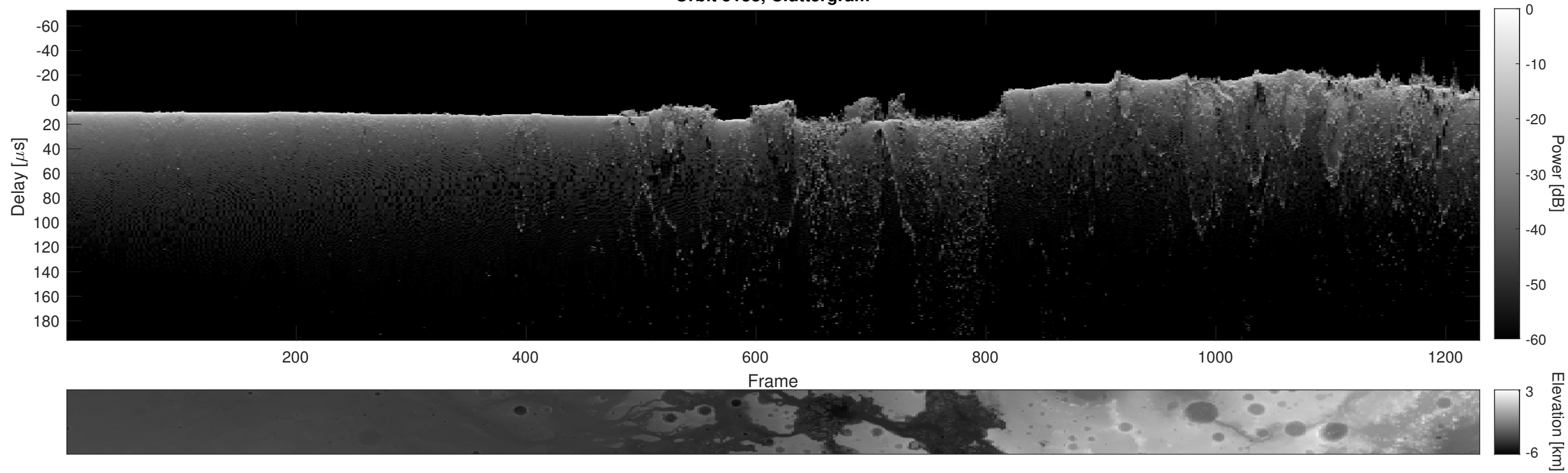
Orbit 5138, Cluttergram
