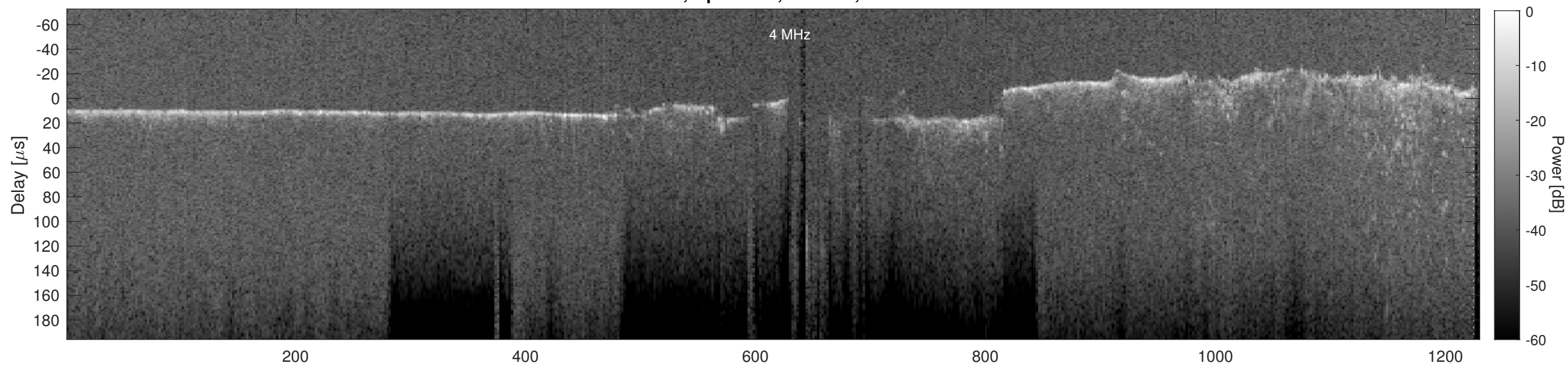
Orbit 5138, Cluttergram
