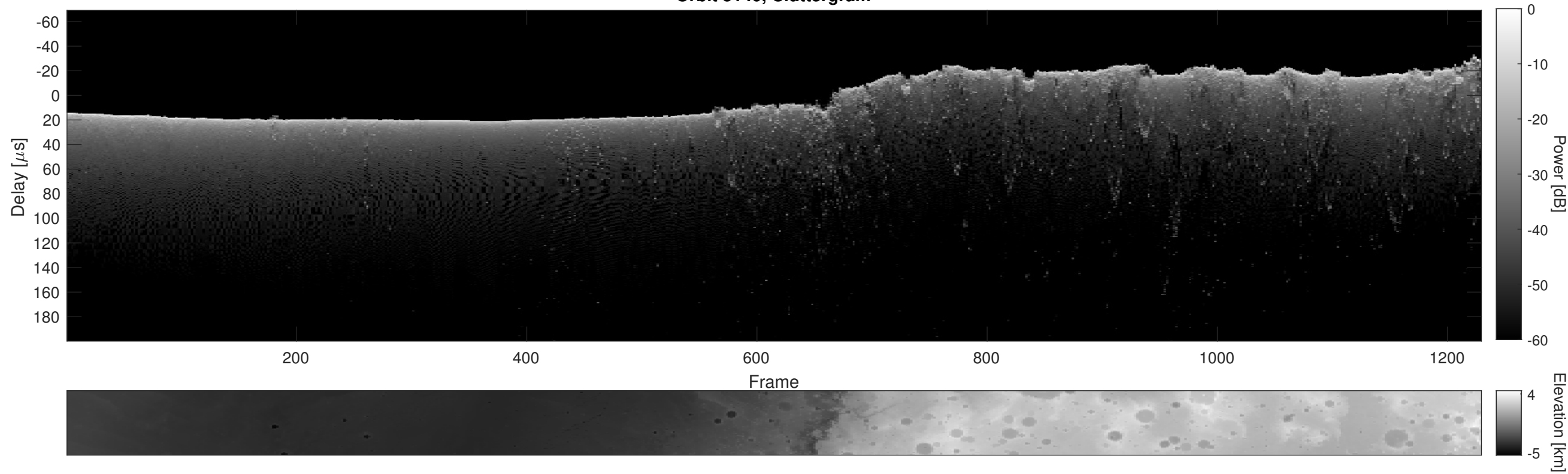
Orbit 5140, Cluttergram
