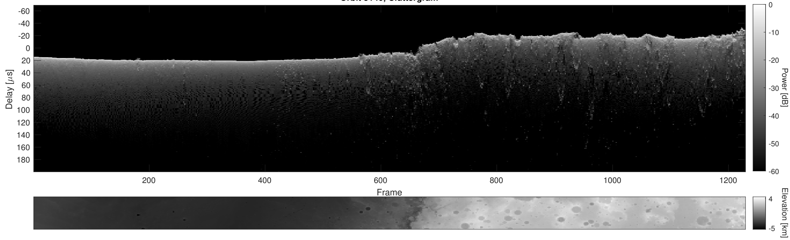
Orbit 5140, Cluttergram
