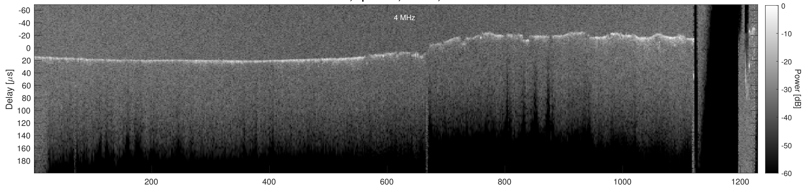
Orbit 5140, Cluttergram
