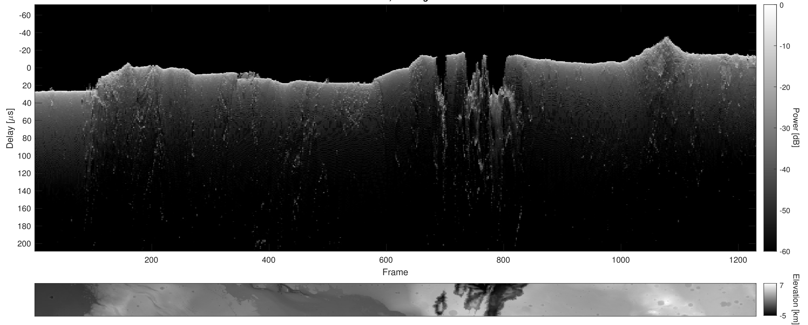
Orbit 5142, Cluttergram
