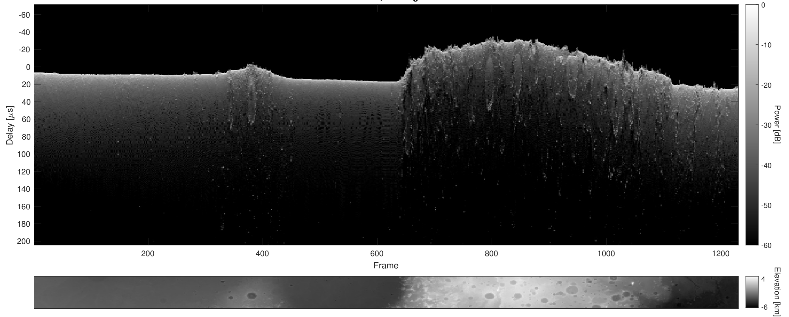
Orbit 5144, Cluttergram
