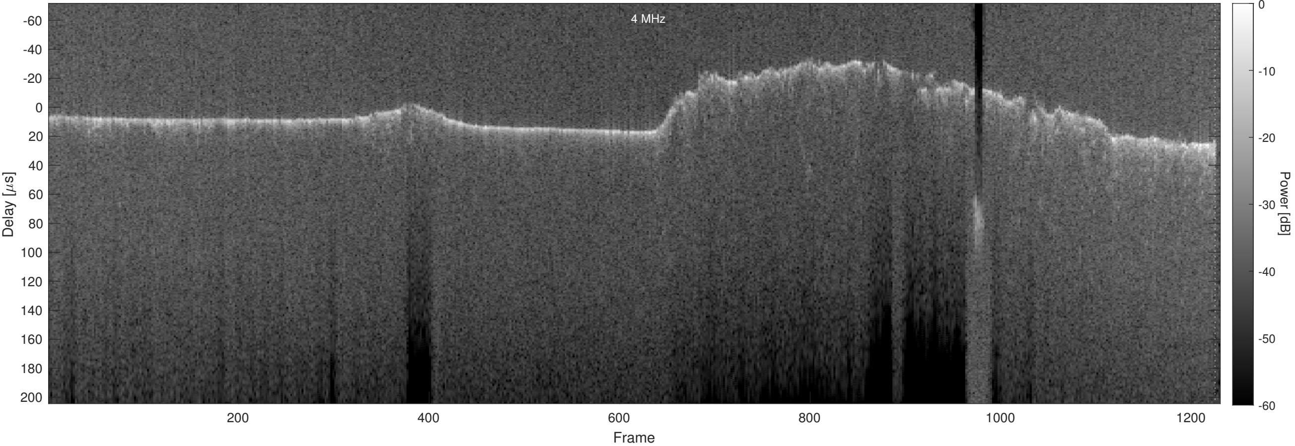
Orbit 5144, Optimized, No Window, Channel 2
