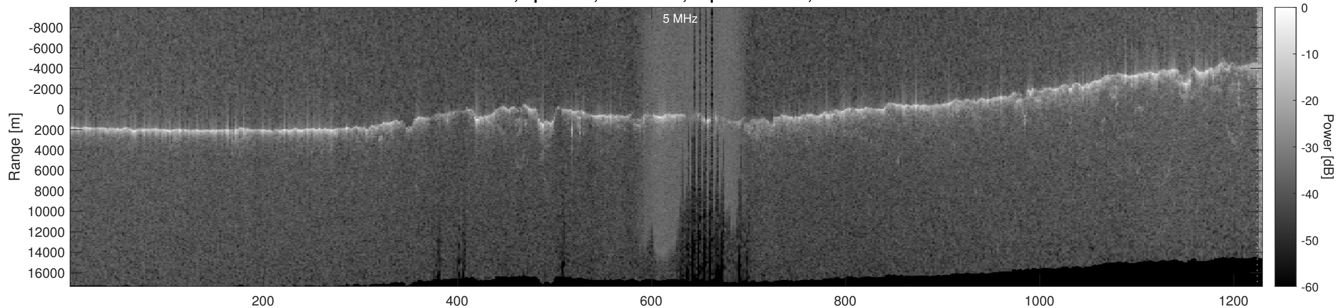
Orbit 5145, Optimized, No Window, Depth-Corrected, Channel 2
