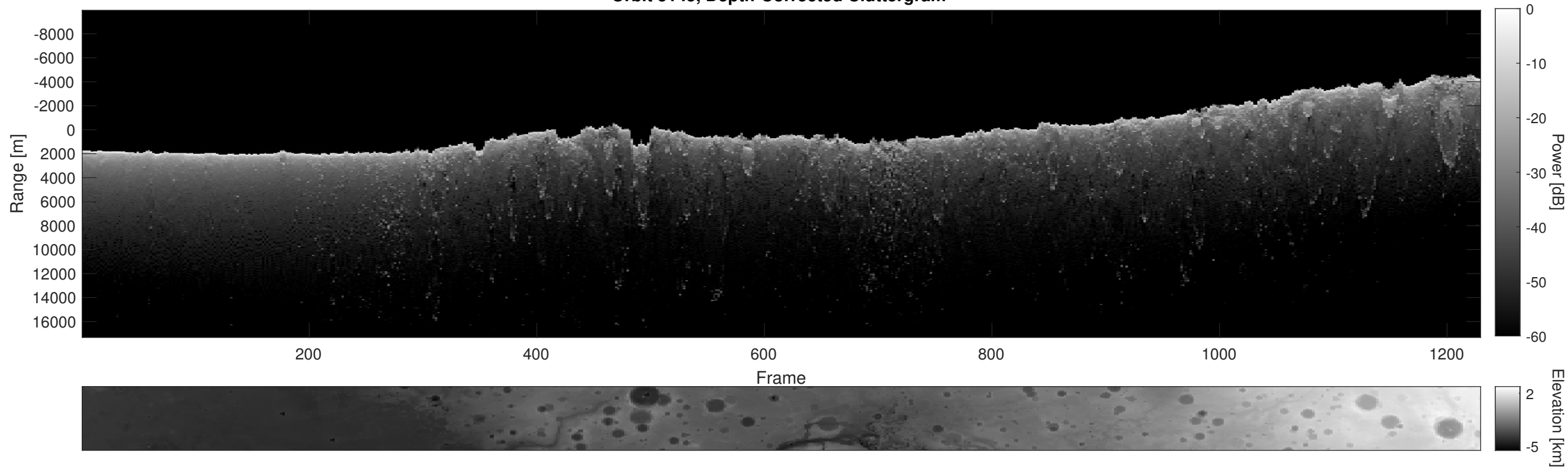
Orbit 5145, Depth-Corrected Cluttergram
