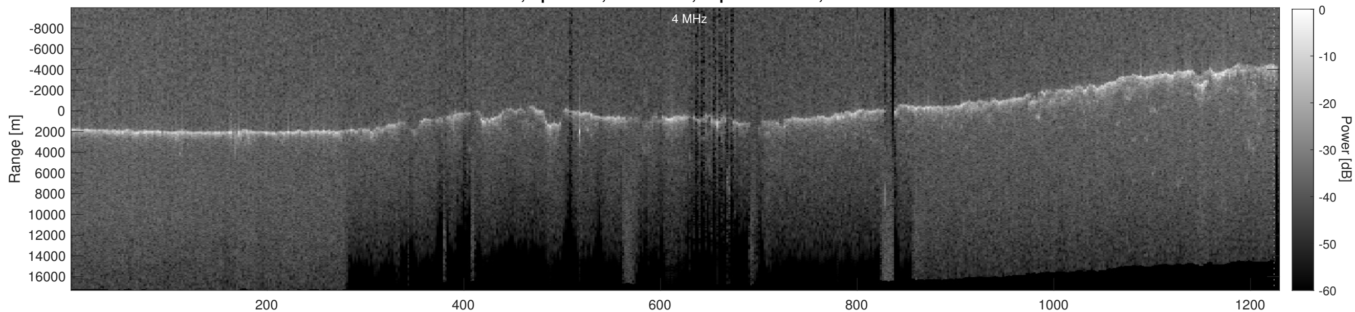
Orbit 5145, Depth-Corrected Cluttergram
