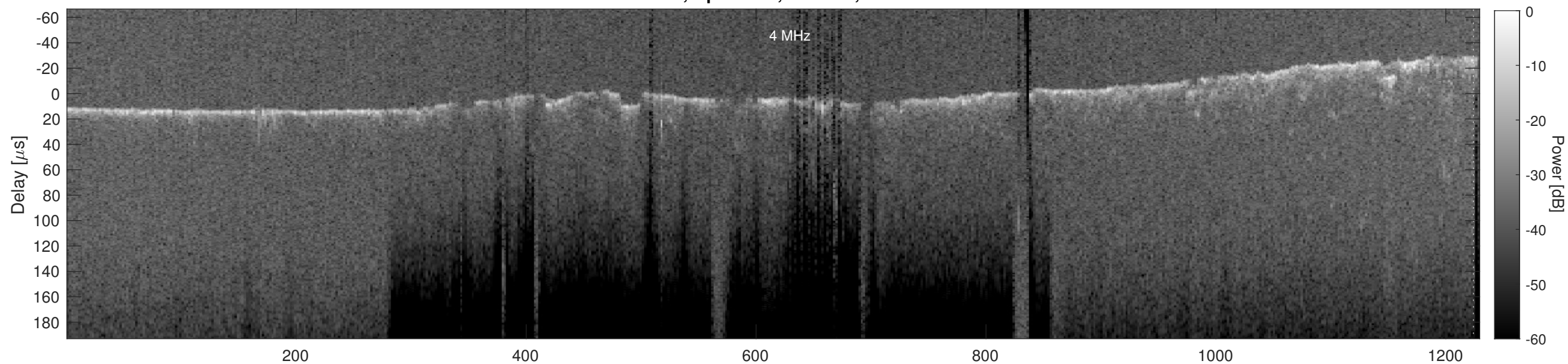
Orbit 5145, Cluttergram
