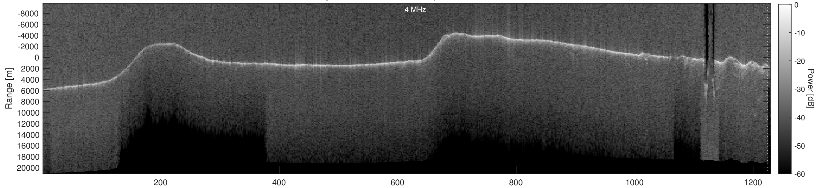
Orbit 5146, Depth-Corrected Cluttergram
