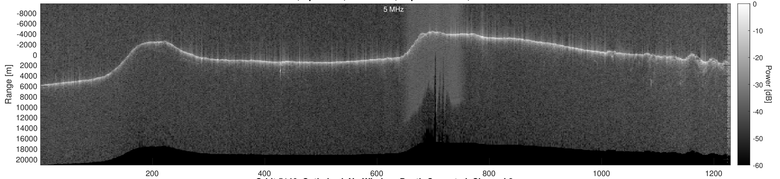
Orbit 5146, Optimized, No Window, Depth-Corrected, Channel 2
