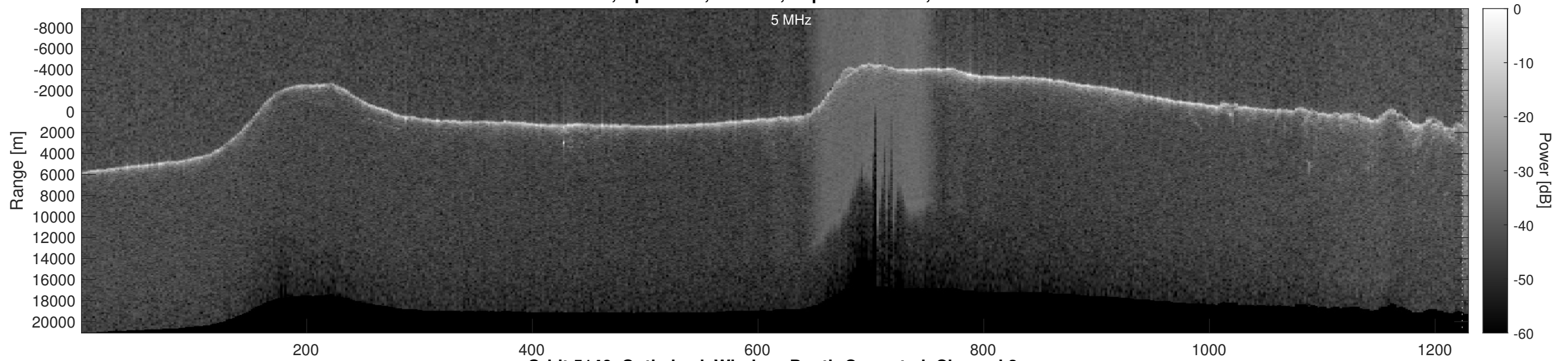
Orbit 5146, Optimized, Window, Depth-Corrected, Channel 2
