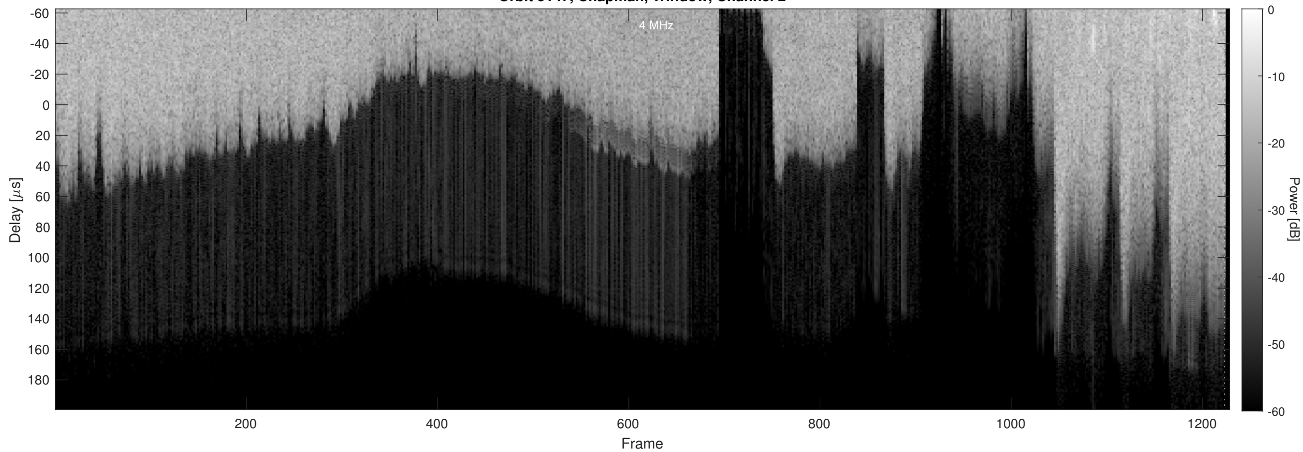
Orbit 5147, Chapman, Window, Channel 2
