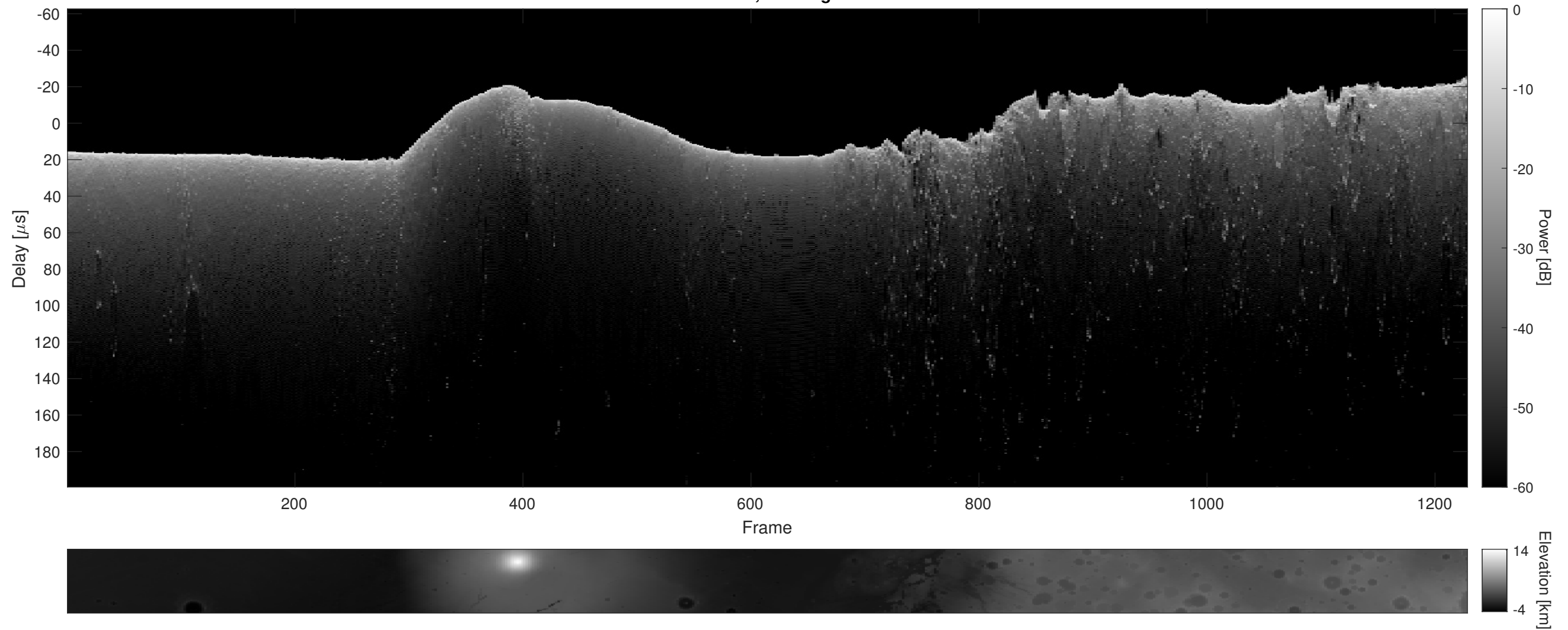
Orbit 5147, Cluttergram
