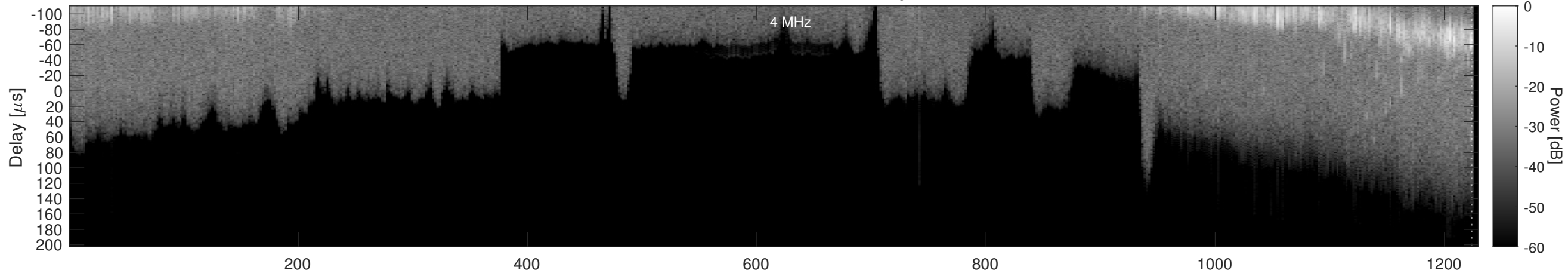
Orbit 5148, Window, Channel 2, Optimized
