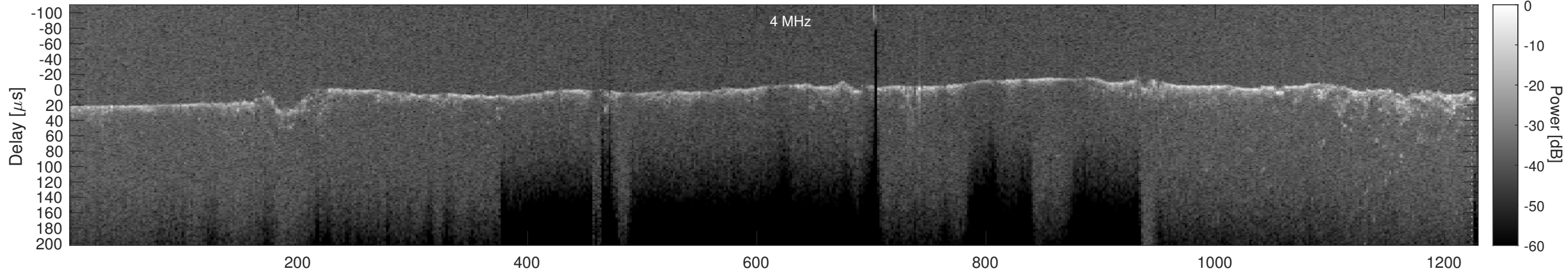
Orbit 5148, Cluttergram
