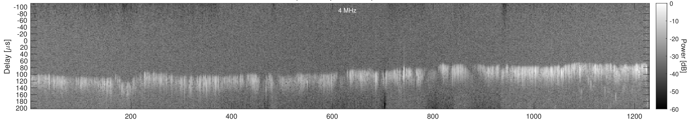
Orbit 5148, Window, Channel 2, Chapman
