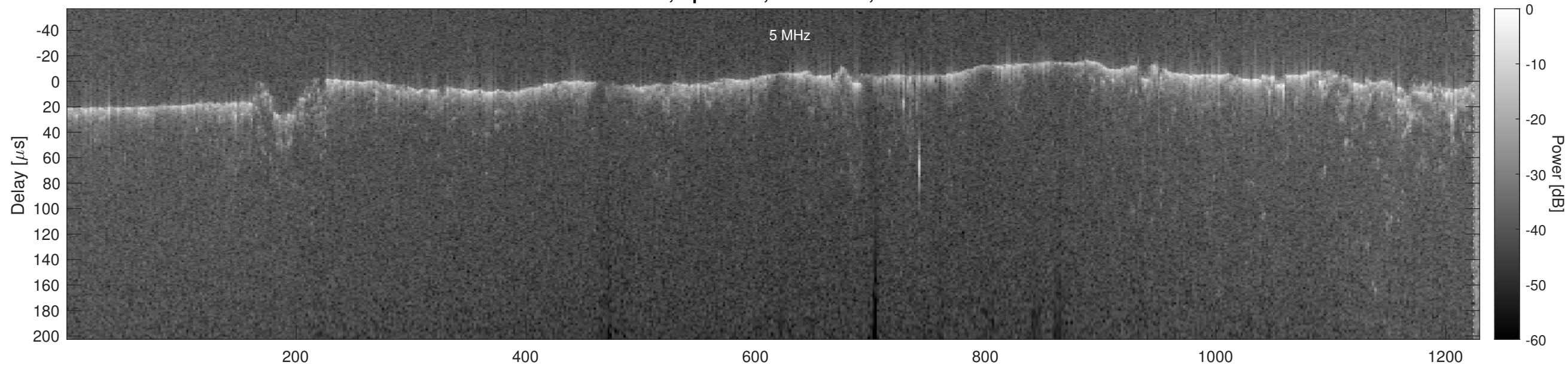
Orbit 5148, Optimized, No Window, Channel 2
