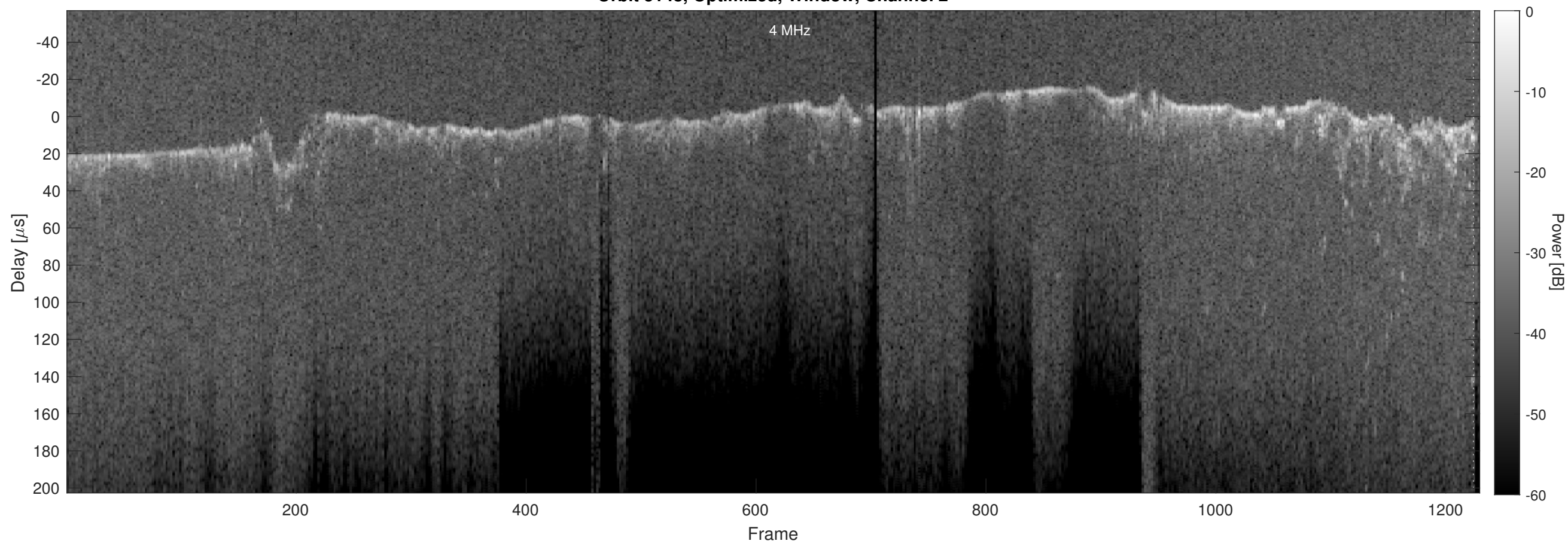
Orbit 5148, Optimized, Window, Channel 2
