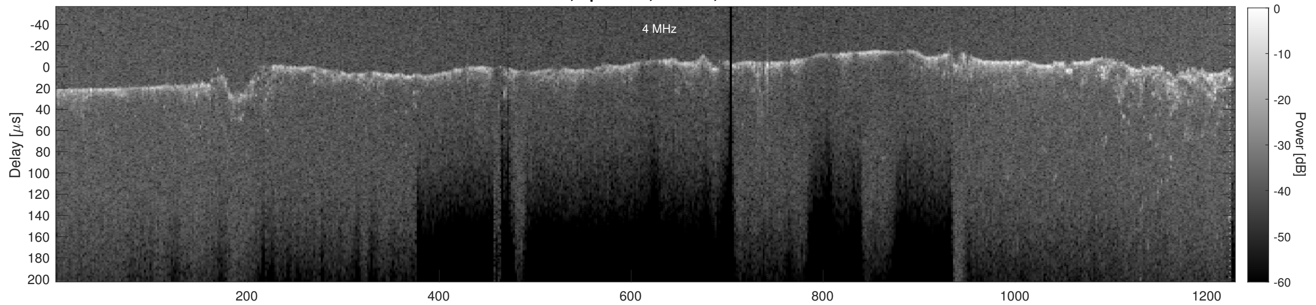
Orbit 5148, Cluttergram
