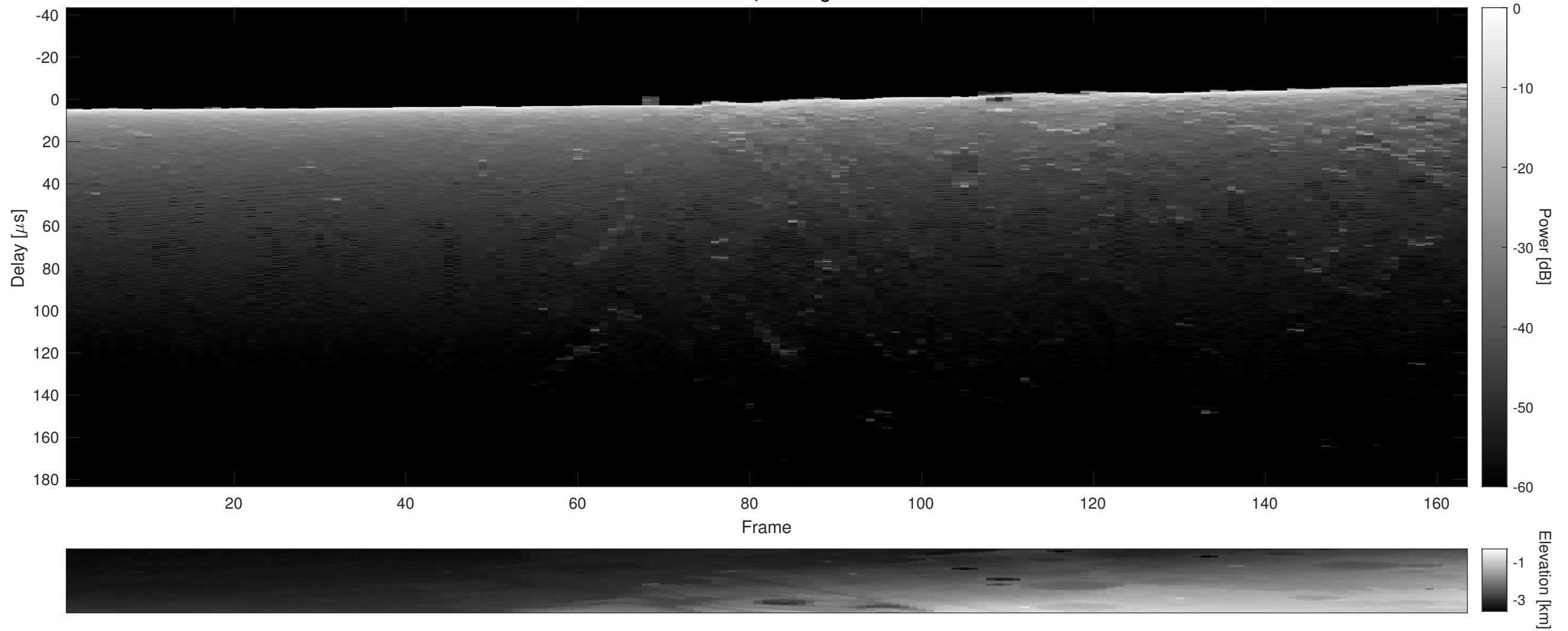
Orbit 5149, Cluttergram
