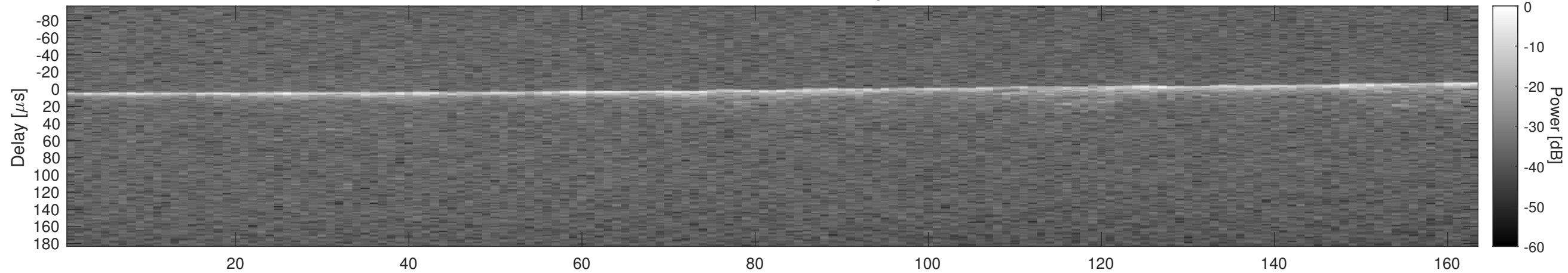
Orbit 5149, Cluttergram
