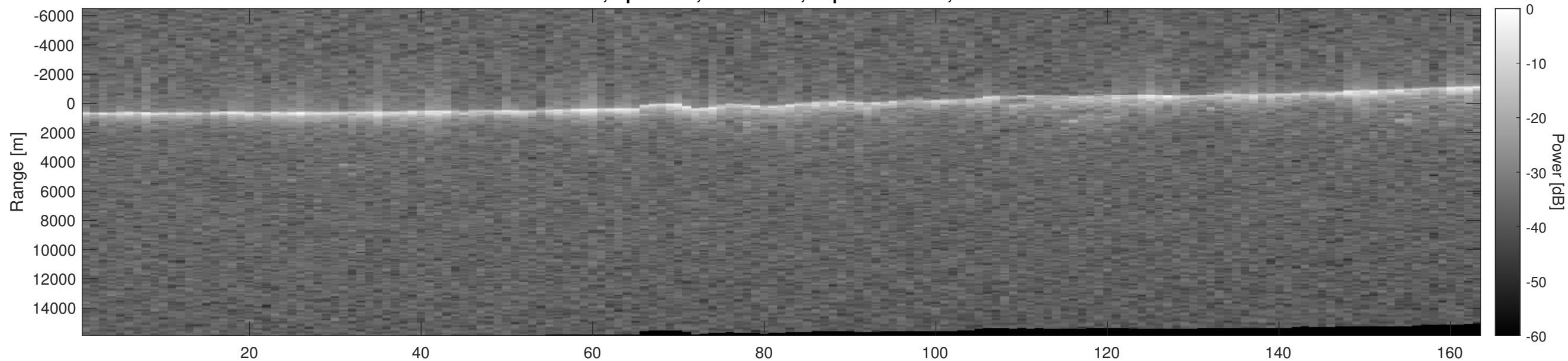
Orbit 5149, Optimized, No Window, Depth-Corrected, Channel 2
