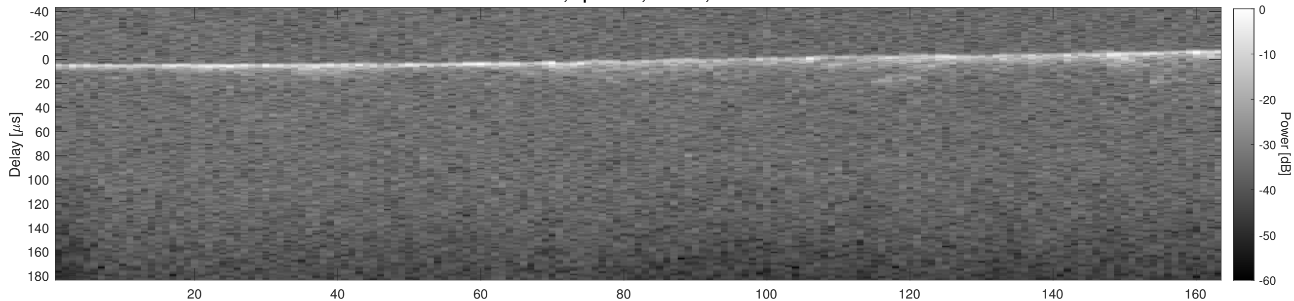
Orbit 5149, Cluttergram
