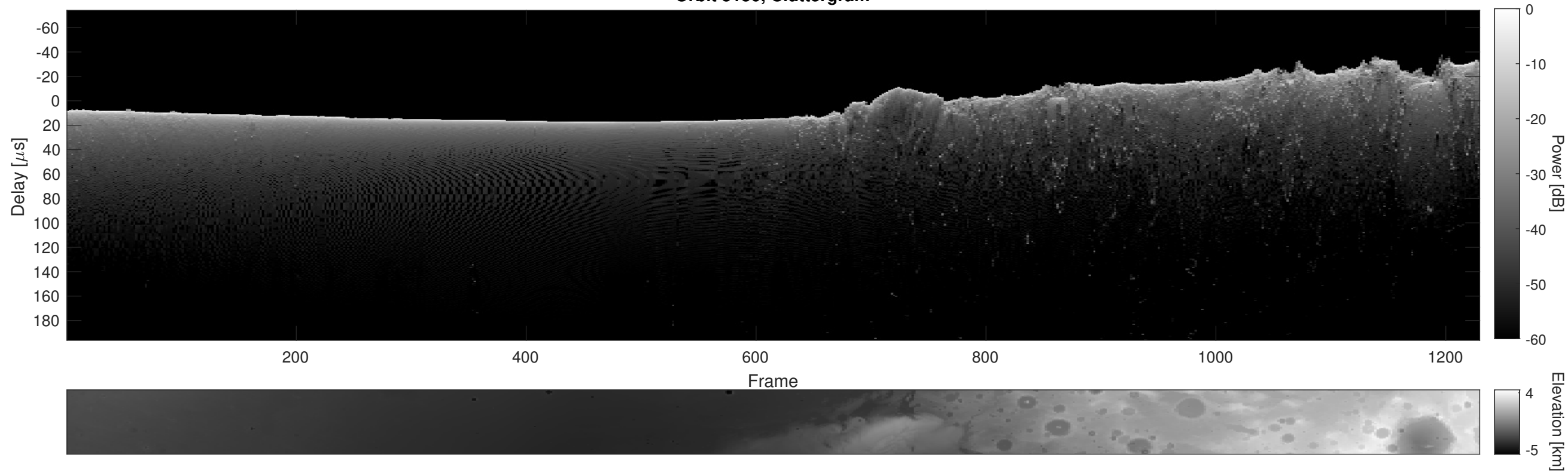
Orbit 5150, Cluttergram
