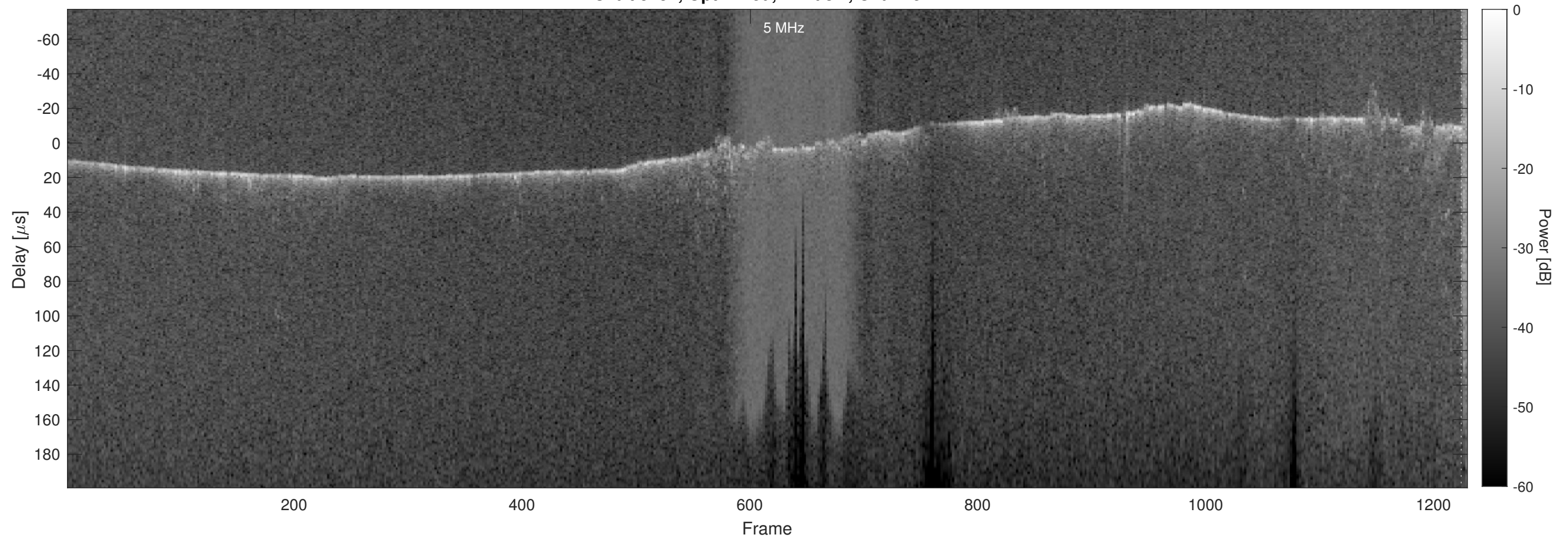
Orbit 5151, Optimized, Window, Channel 2
