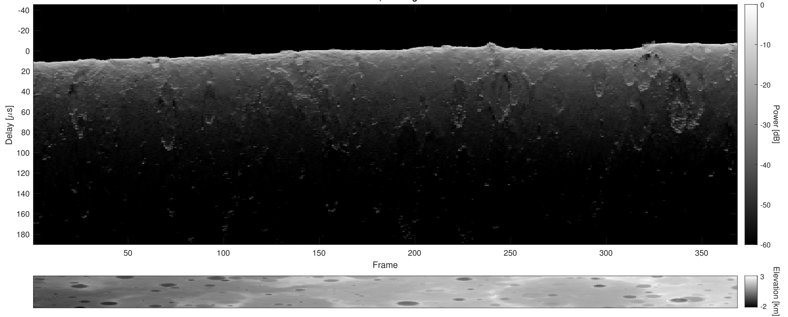
Orbit 5152, Cluttergram
