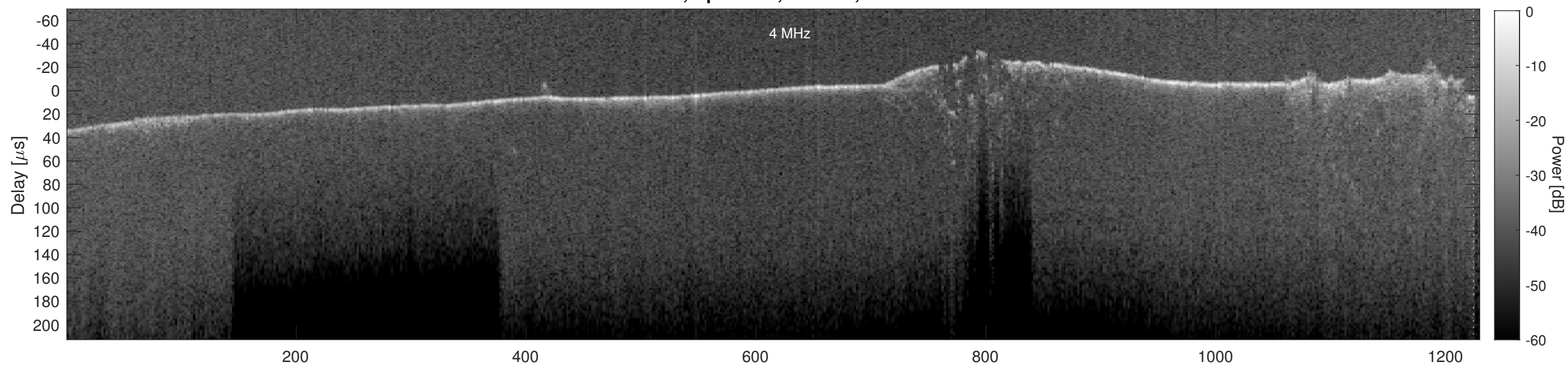
Orbit 5153, Cluttergram
