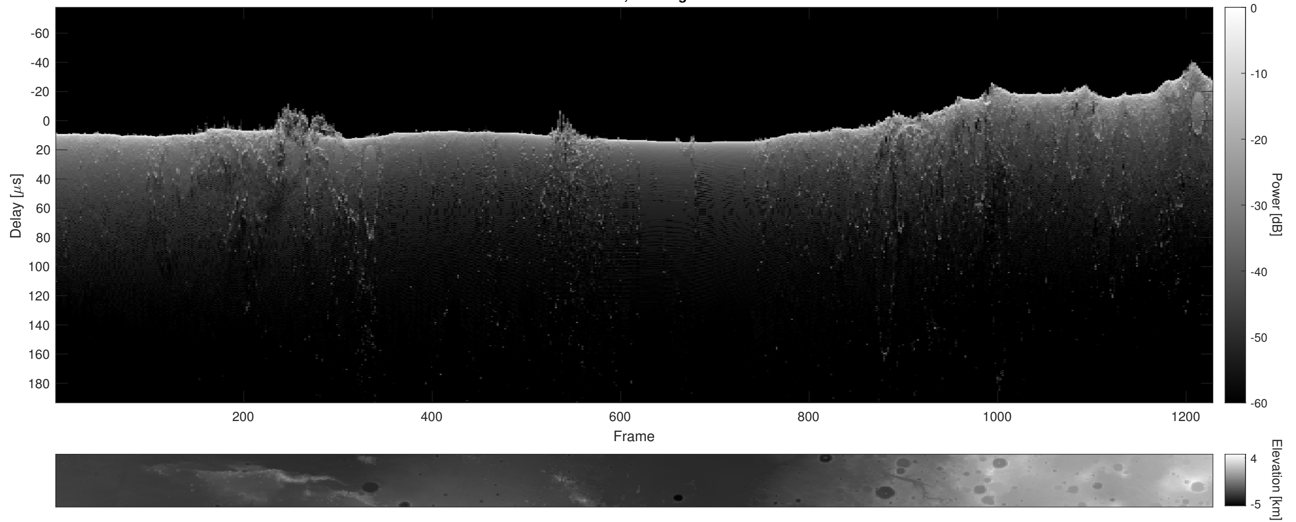
Orbit 5154, Cluttergram
