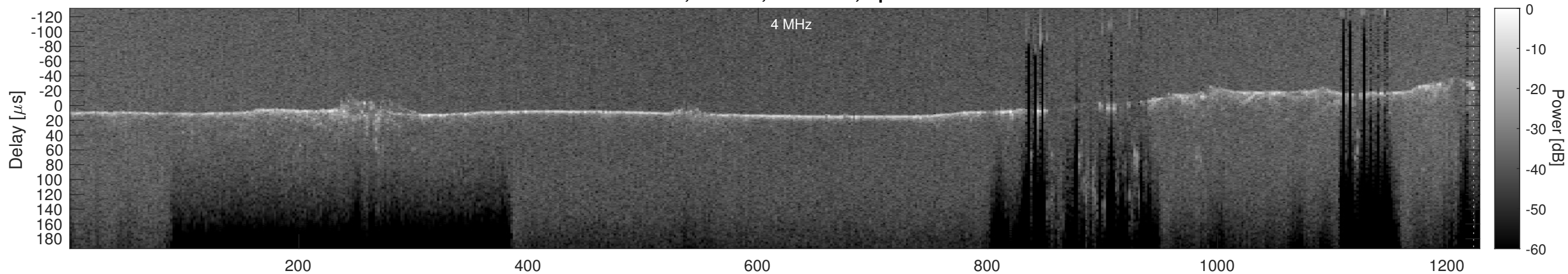
Orbit 5154, Cluttergram
