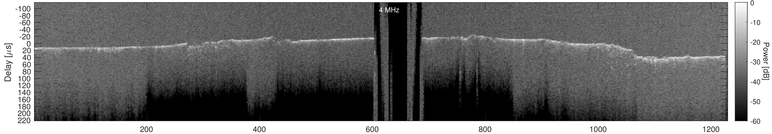
Orbit 5155, Cluttergram
