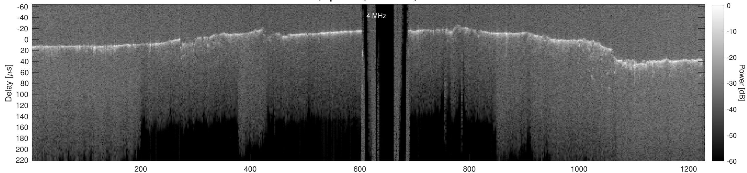
Orbit 5155, Cluttergram
