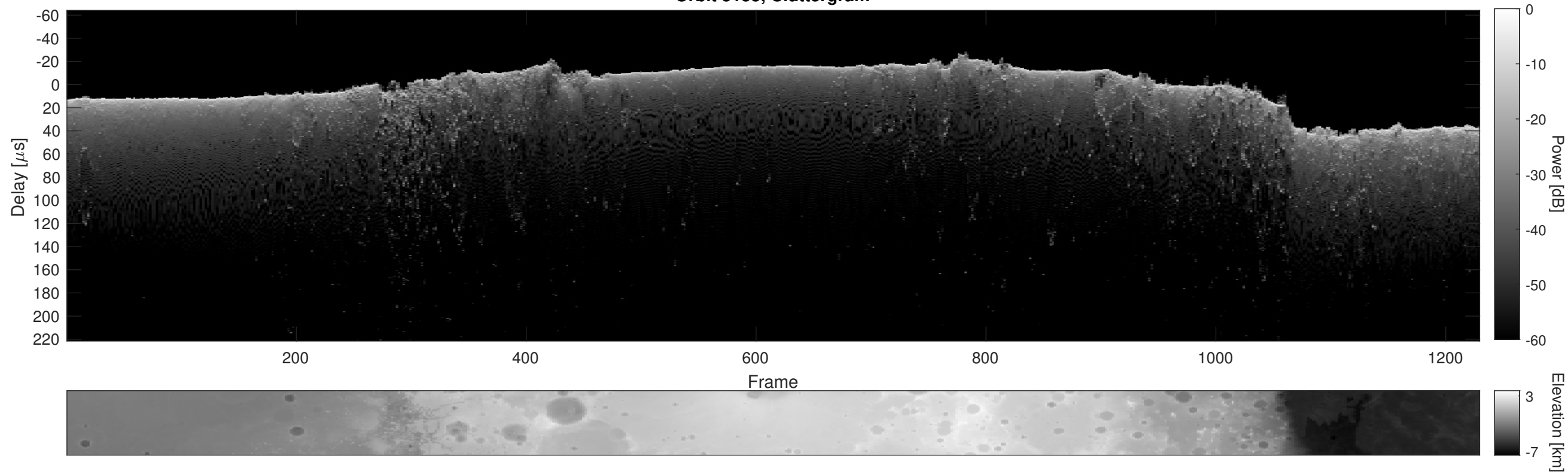
Orbit 5155, Cluttergram
