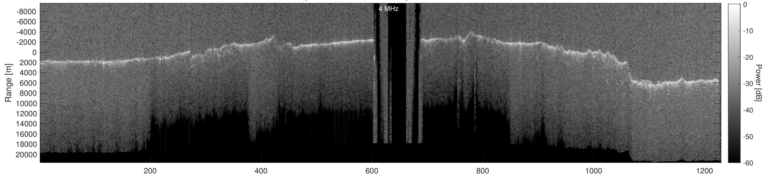
Orbit 5155, Depth-Corrected Cluttergram
