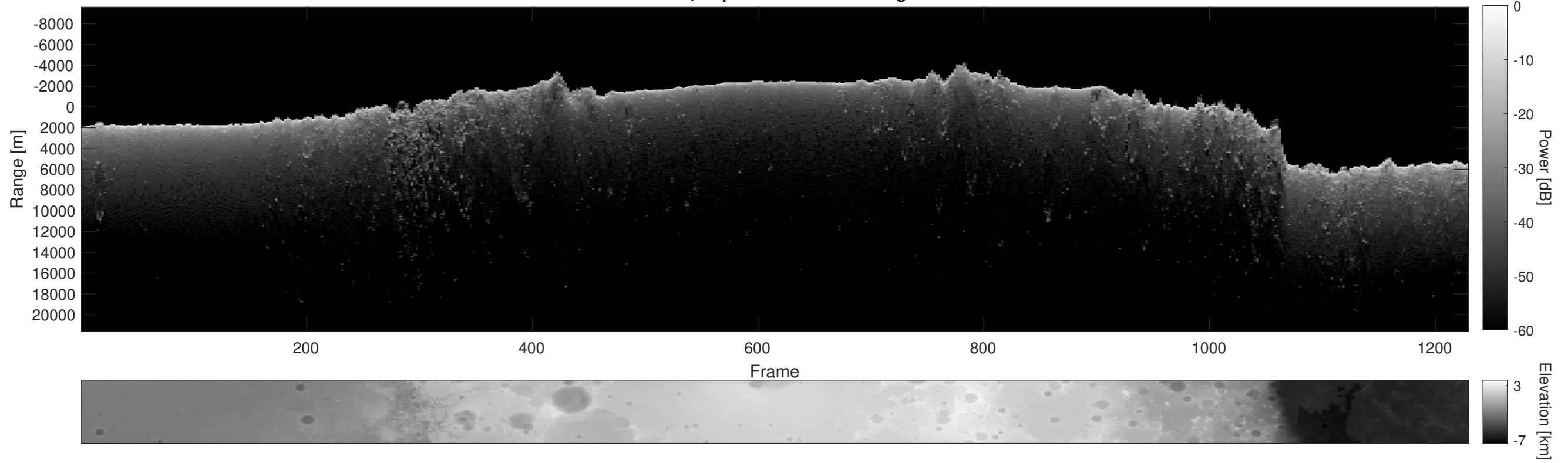
Orbit 5155, Depth-Corrected Cluttergram
