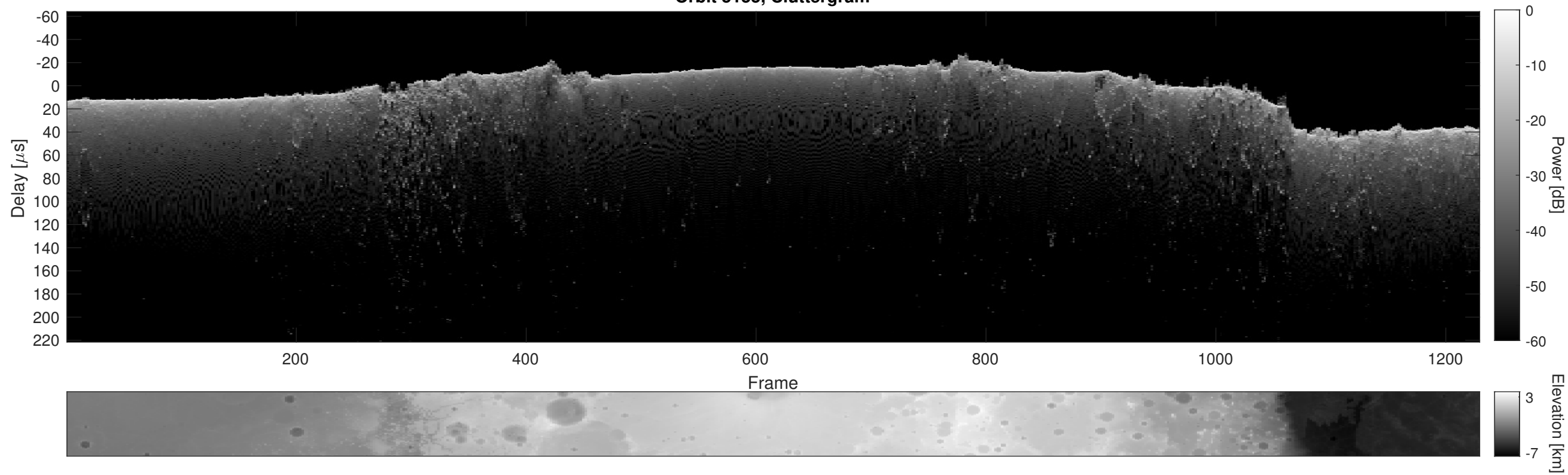
Orbit 5155, Cluttergram
