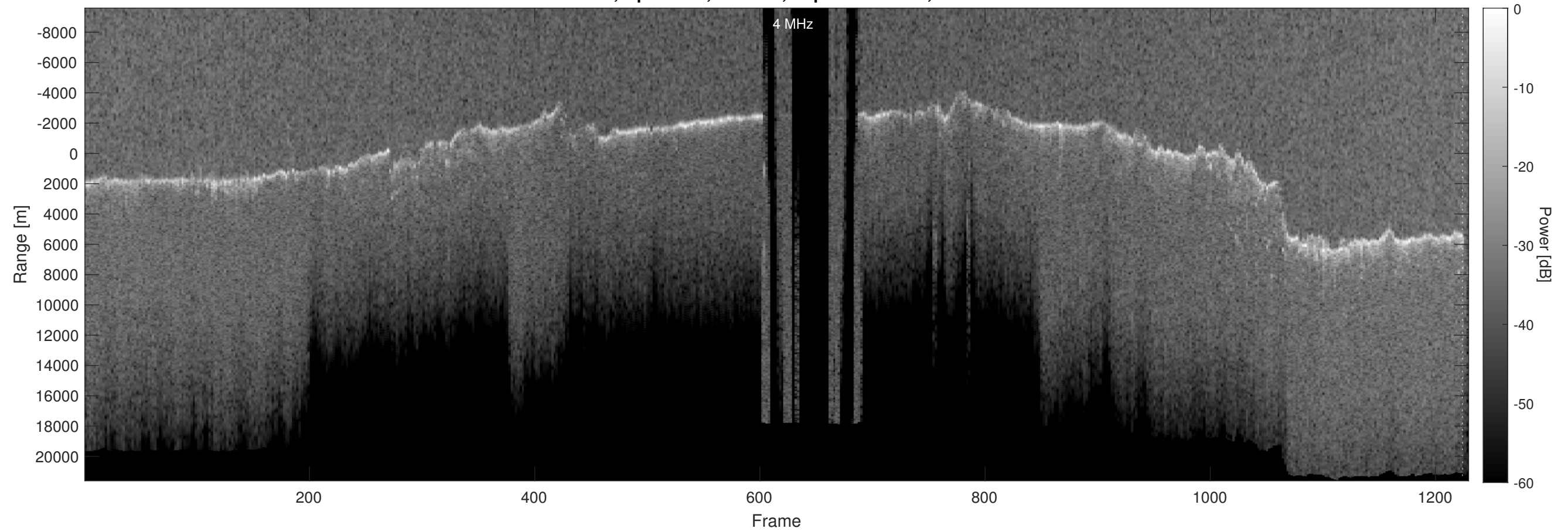
Orbit 5155, Optimized, Window, Depth-Corrected, Channel 2
