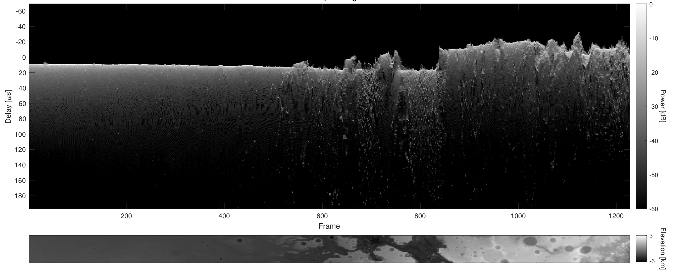
Orbit 5156, Cluttergram
