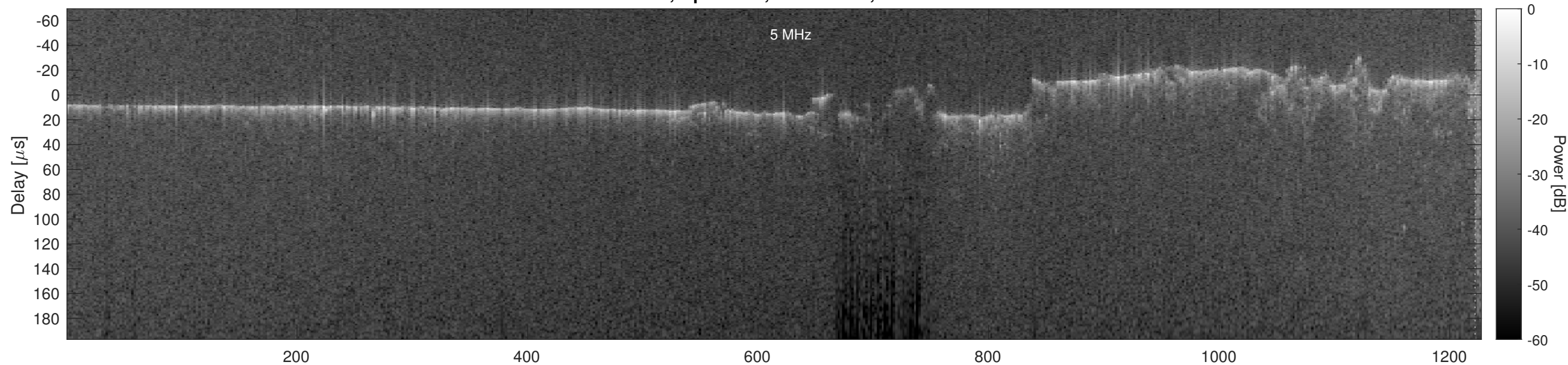
Orbit 5156, Optimized, No Window, Channel 2
