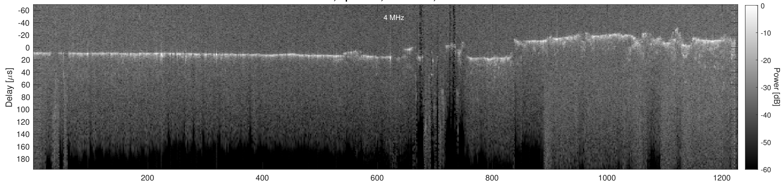
Orbit 5156, Cluttergram
