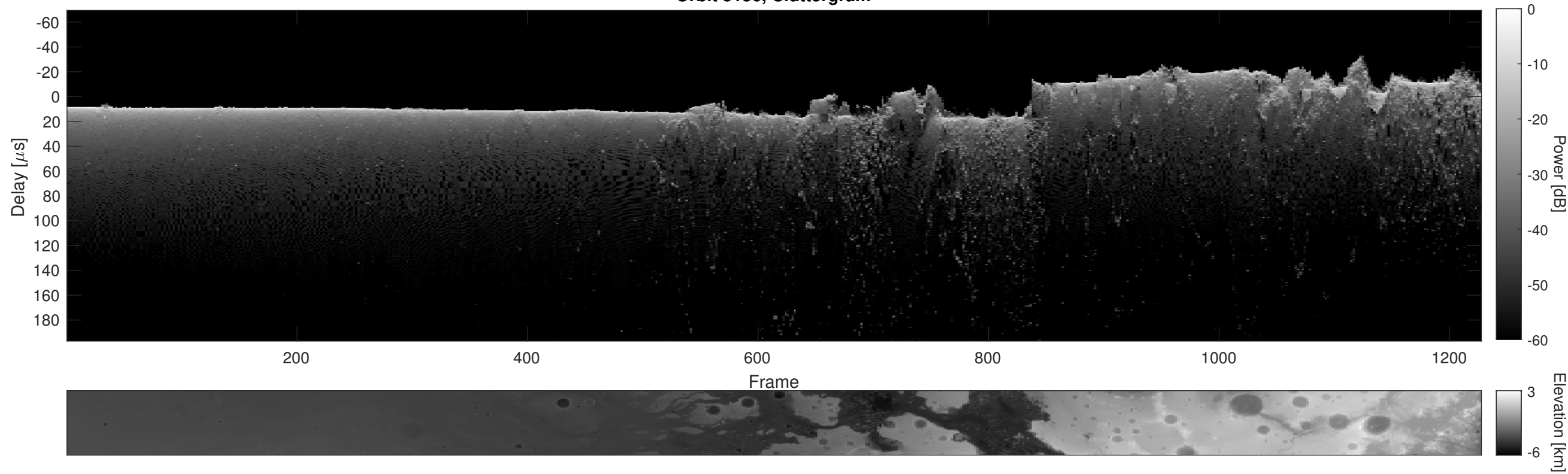
Orbit 5156, Cluttergram
