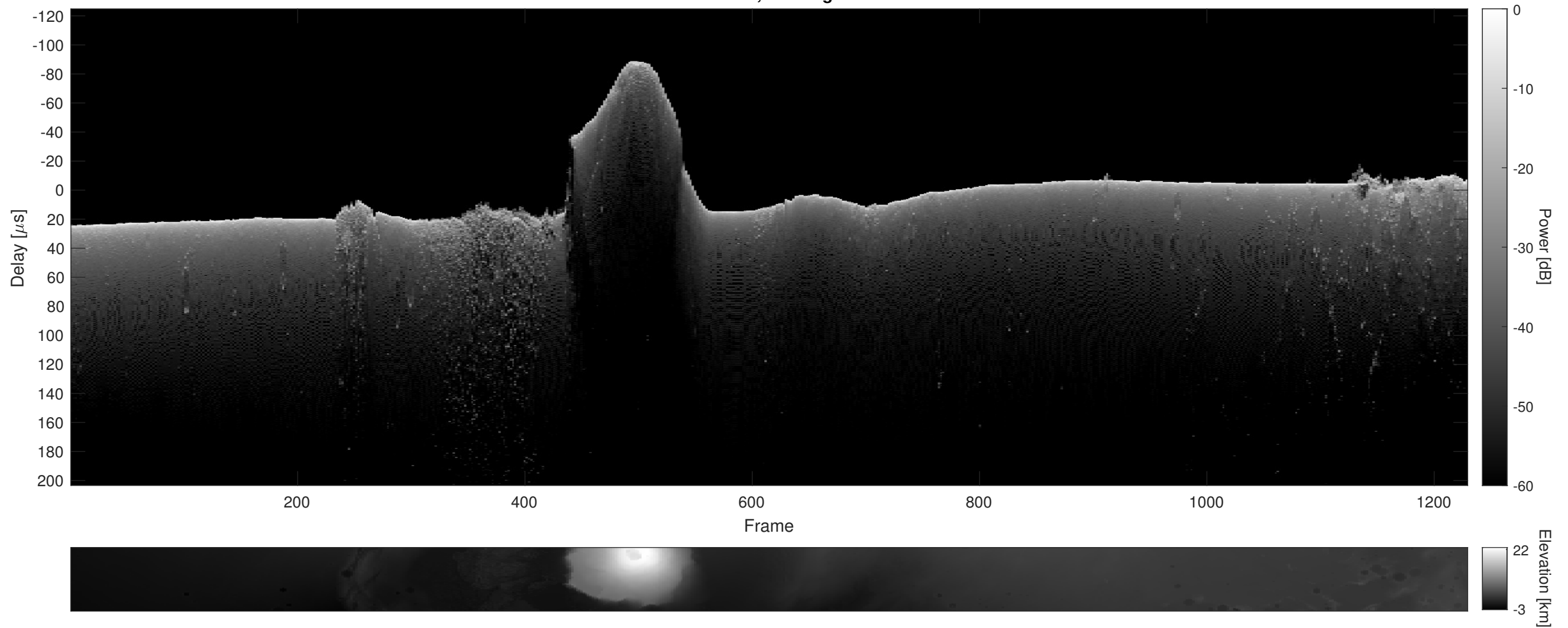
Orbit 5157, Cluttergram
