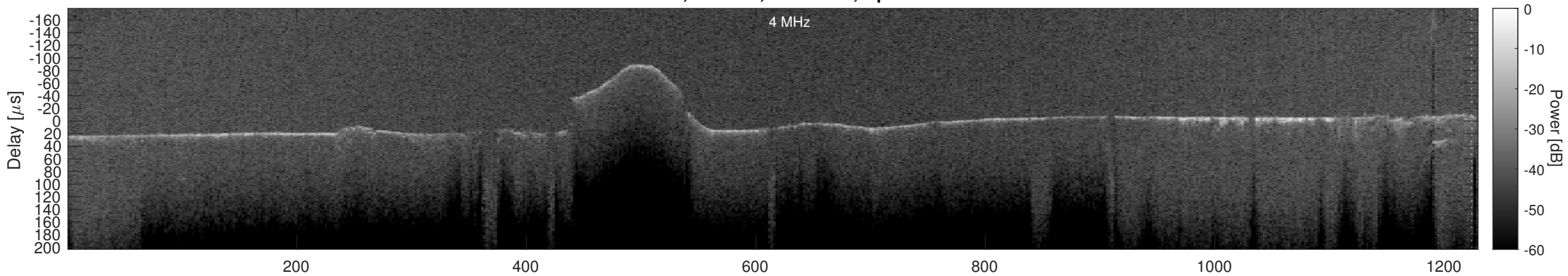
Orbit 5157, Cluttergram
