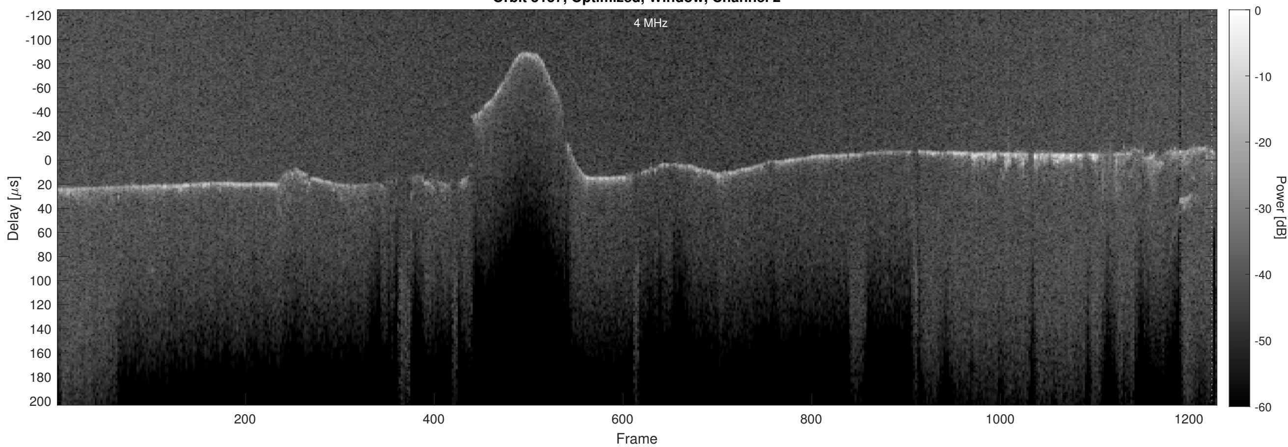
Orbit 5157, Optimized, Window, Channel 2
