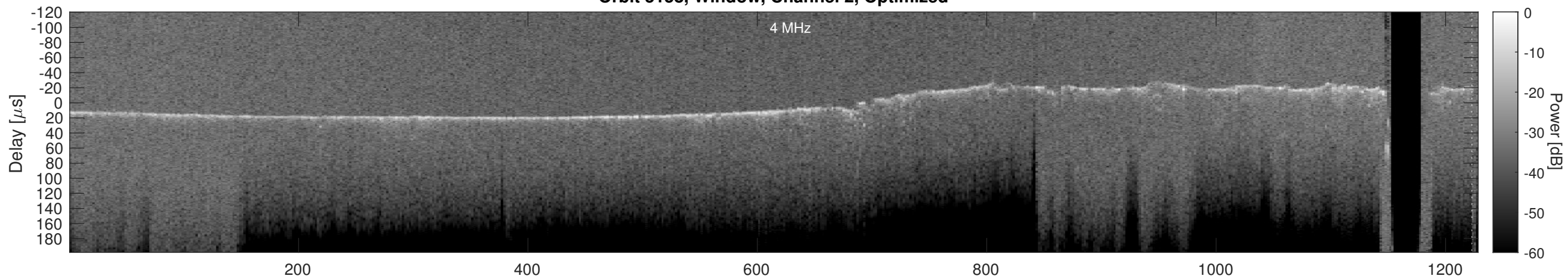
Orbit 5158, Cluttergram
