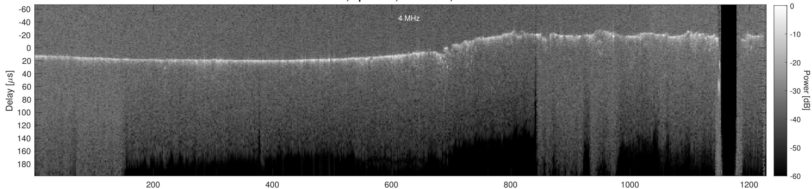
Orbit 5158, Cluttergram
