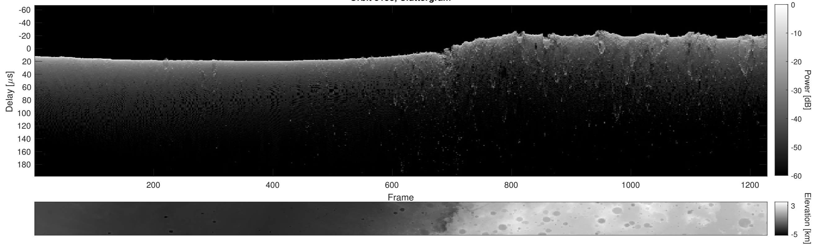
Orbit 5158, Cluttergram
