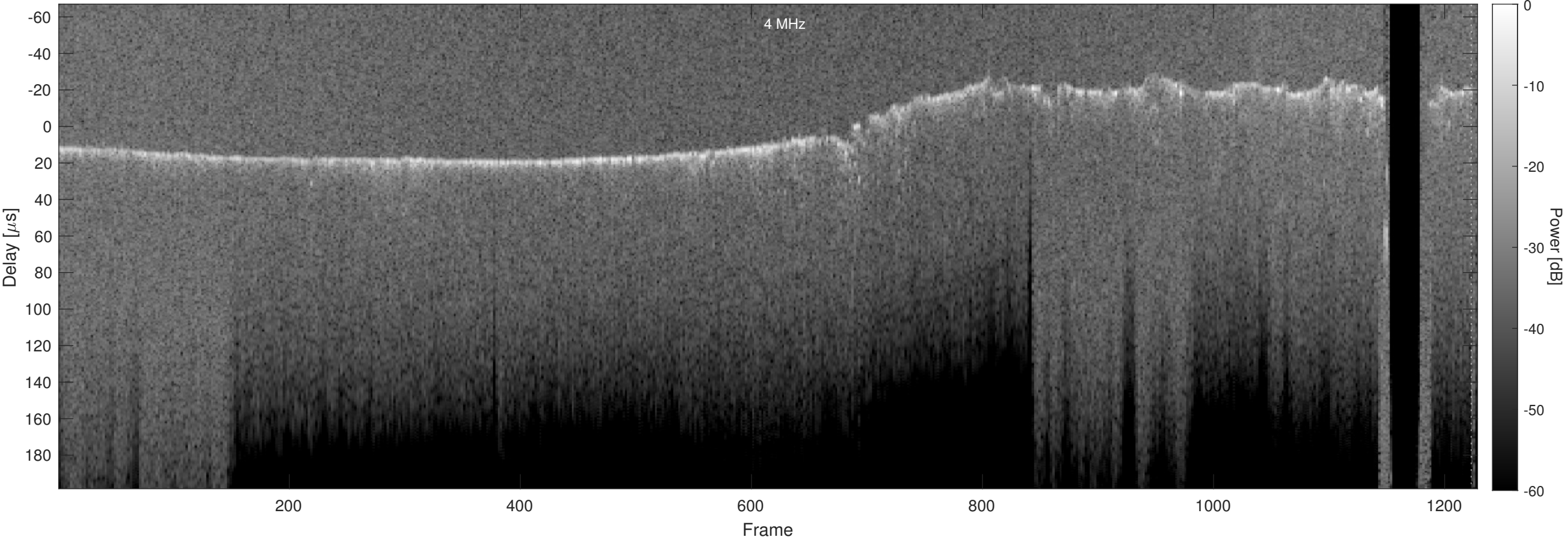
Orbit 5158, Optimized, Window, Channel 2
