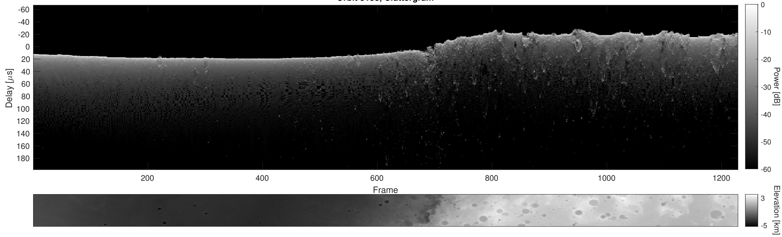
Orbit 5158, Cluttergram
