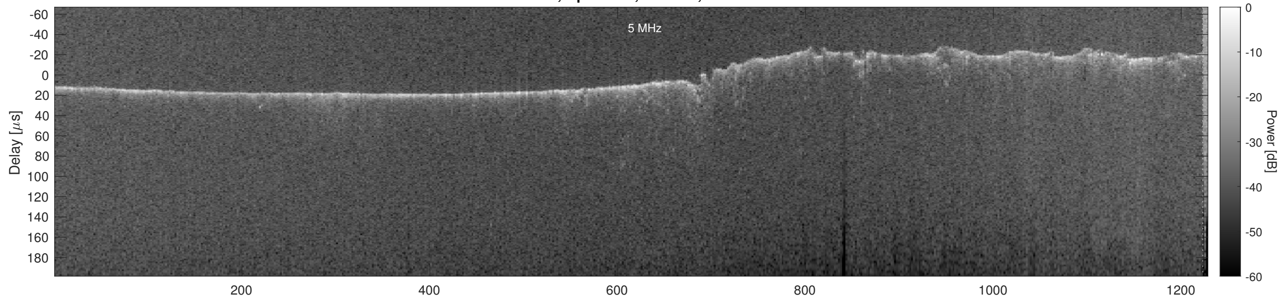
Orbit 5158, Optimized, Window, Channel 2
