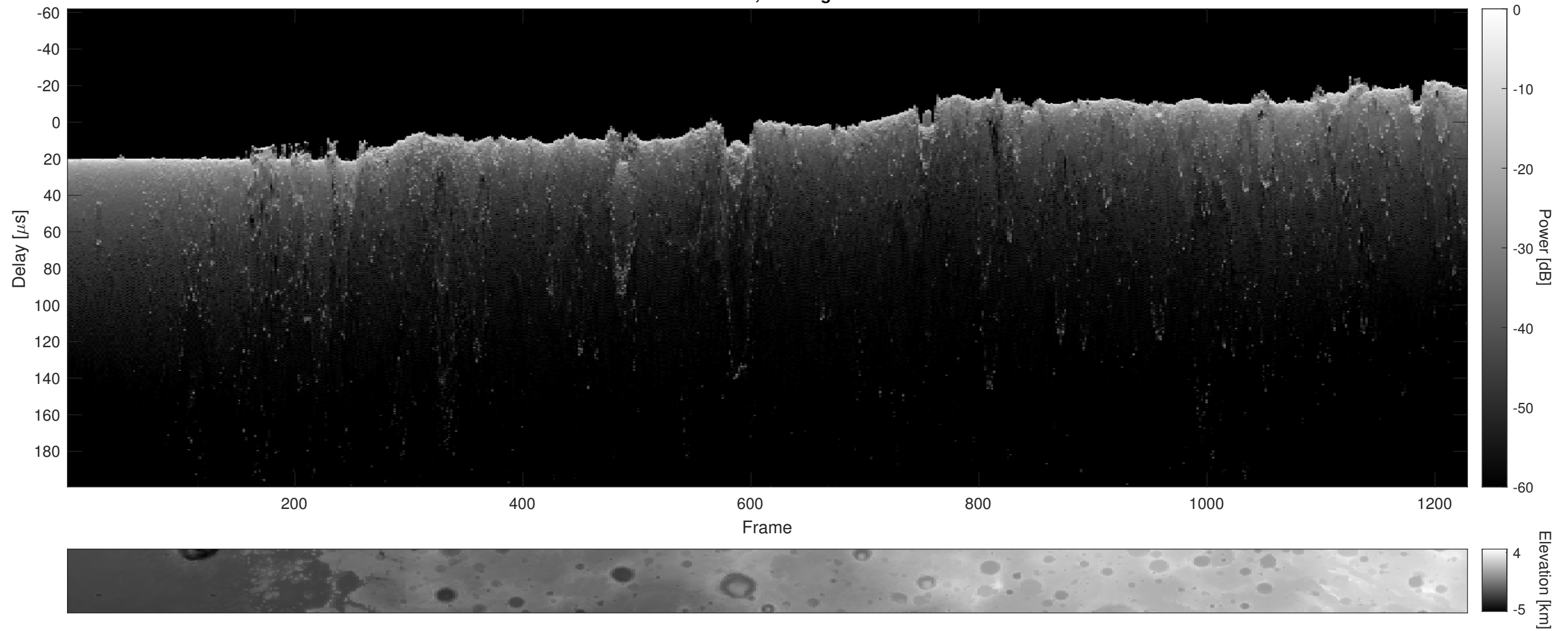
Orbit 5159, Cluttergram
