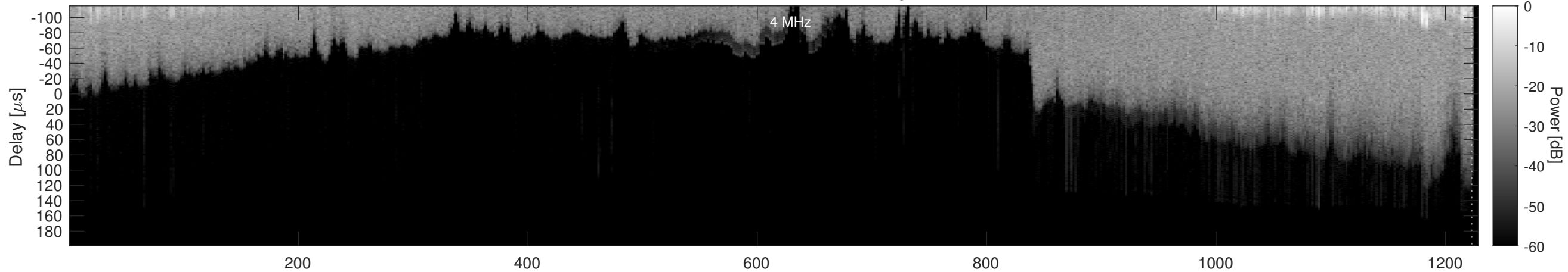
Orbit 5159, Window, Channel 2, Optimized
