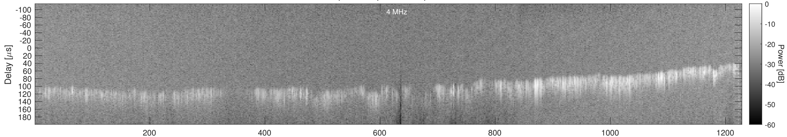
Orbit 5159, Window, Channel 2, Chapman
