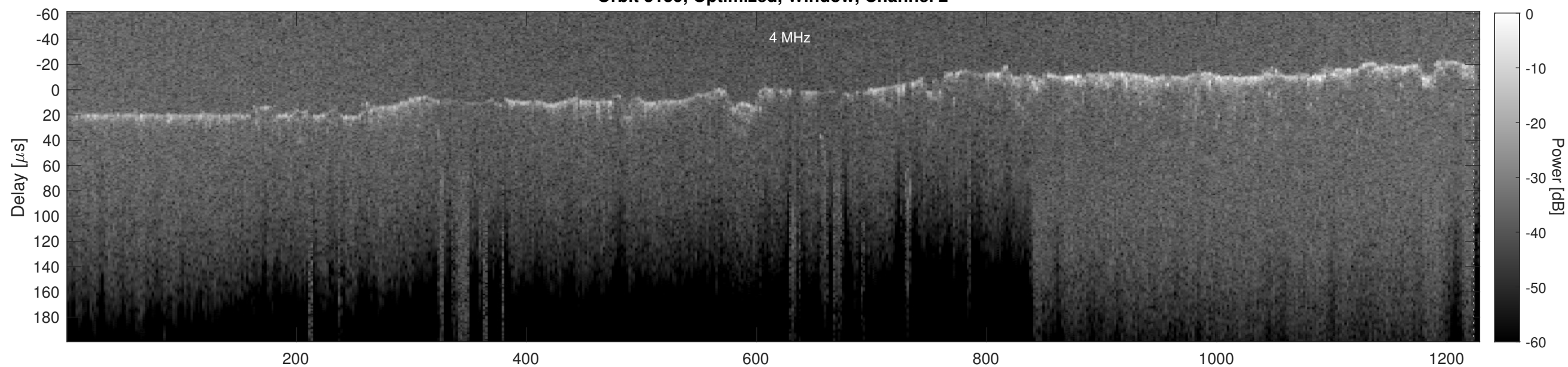
Orbit 5159, Cluttergram
