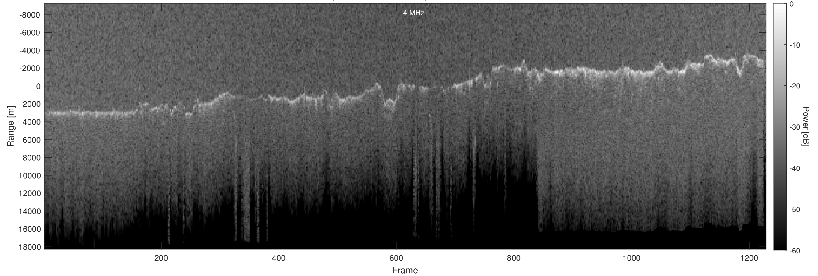
Orbit 5159, Optimized, Window, Depth-Corrected, Channel 2
