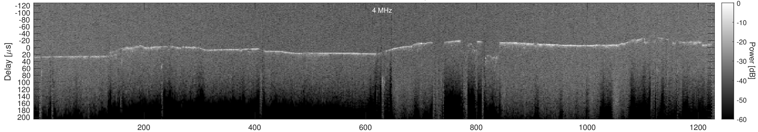
Orbit 5160, Cluttergram
