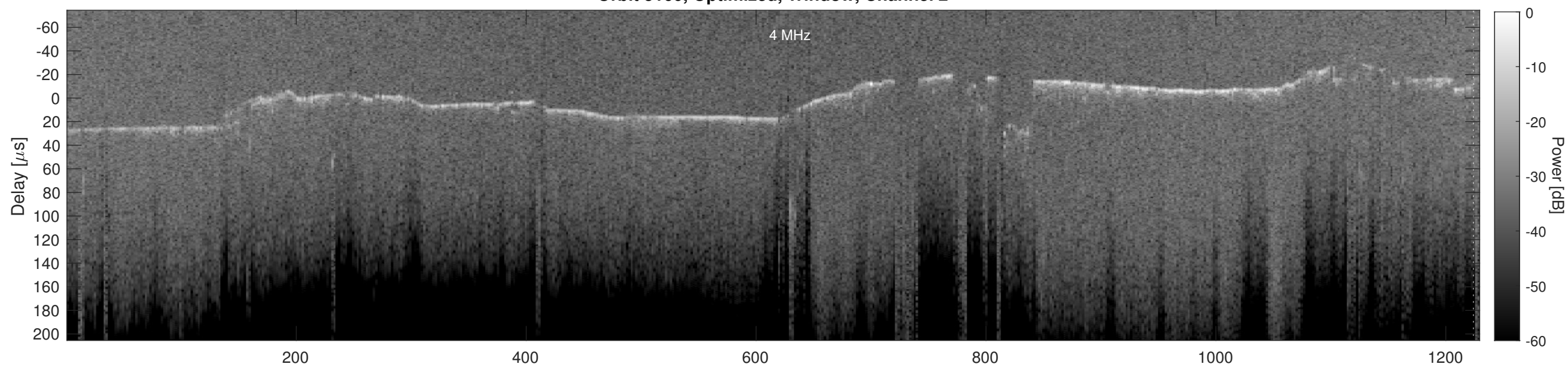
Orbit 5160, Cluttergram
